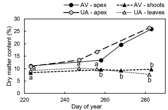
FIGURE 4 Dry matter content of shoot apices and young leaves/shoots in summer growing plants and developing turions of the three stages in A. vesiculosa and U. australis . Means \pm SE intervals are shown for leaves/shoots, n = 4 . Different letters for one parameter and species denote statistically significant difference at P < .05 . Day of year 223 is August 11 (start of the experiment).
