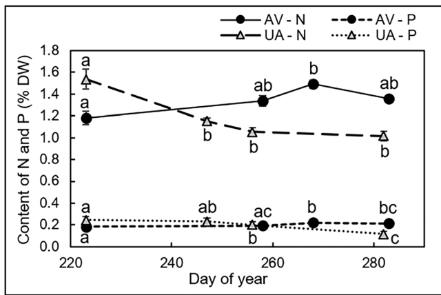
FIGURE 3 Content of N or P in young leaves/shoots of A. vesiculosa and U. australis in summer growing plants and developing turions of the three stages. Means \pm SE intervals, n = 5 . Different letters for one parameter and species denote statistically significant difference at P < .05 . Day of year 2023 is August 11 (start of the experiment).
