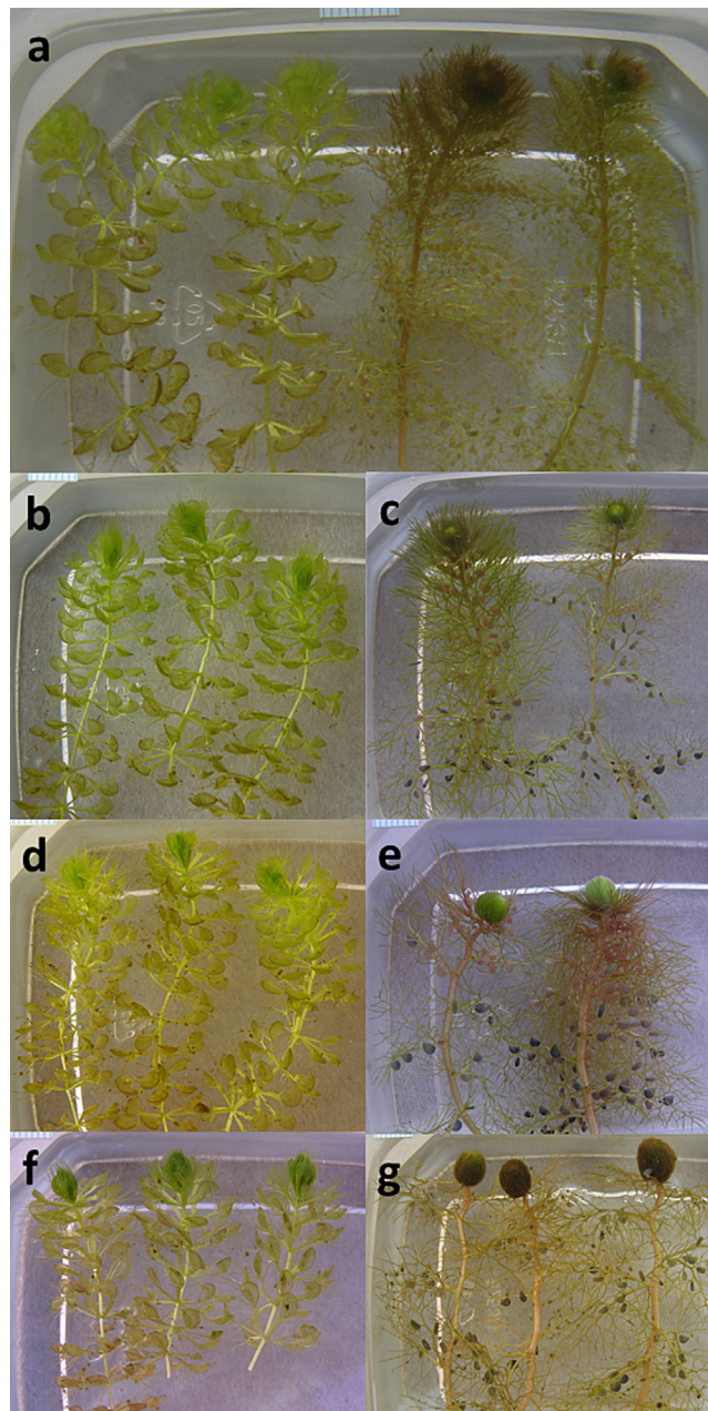
FIGURE 1 Photos of summer growing plants (a) of Aldrovanda vesiculosa (left) and Utricularia australis (right) and three arbitrary stages of turion development. (b, c) Stage I, first symptoms of turion development; (d, e) Stage II, turion ripening; (f, g) Stage III, morphological turion maturity. The ticks on the top of sections denote 1 mm. For details, see the text and Table S1.
